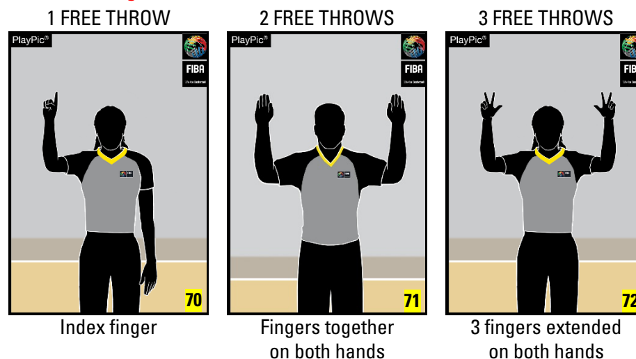
Diagram 8 Referees' signals
